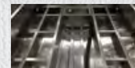
LONGITUDINAL STRUCTURE 6 beams in total with 3 on each side of center
